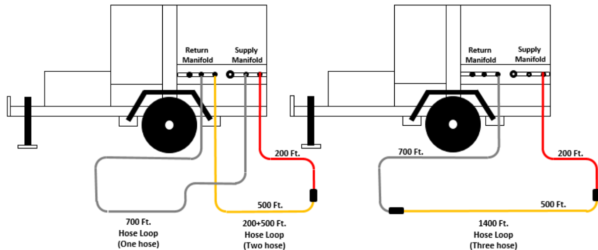
Two-Zone configuration using 700 Ft. hose per zone (Preferred method)
